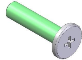
FLAT HEAD BOLT (M5X25L) – 12EA
