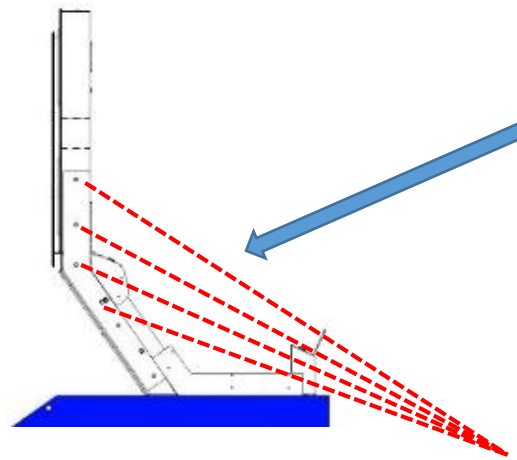
BILLBOARD Ass'y SIDE SUPPORT BRKT (2EA)
