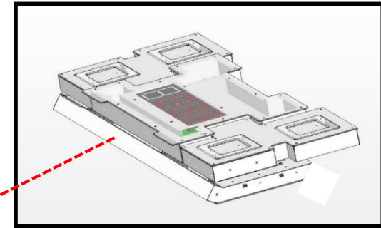
BILLBOARD Ass'y (1EA)
