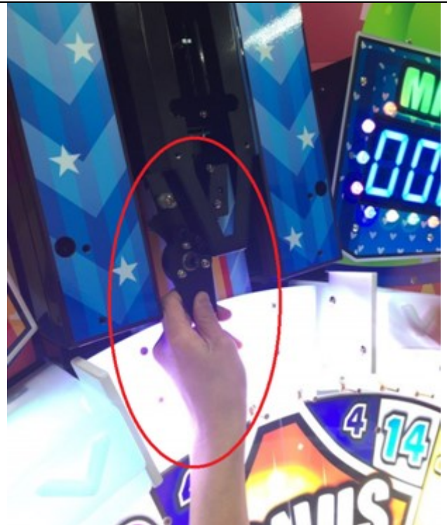
4. Replace new dropping arrow assembly.
